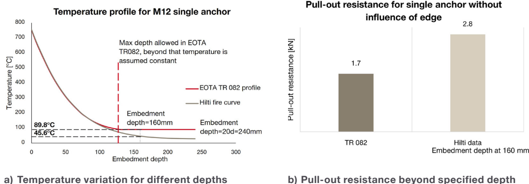
Fig. 6.45: Comparison between EOTA TR 082 [46] and Hilti developed data for a threaded rod M12
