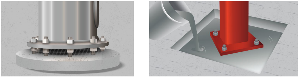
a) Ungrooved stand-off connection: in service b) Installation of flowable grout in recessed column base
