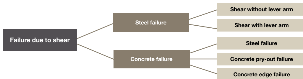
Fig. 3.14: Different types of failures due to shear loading
