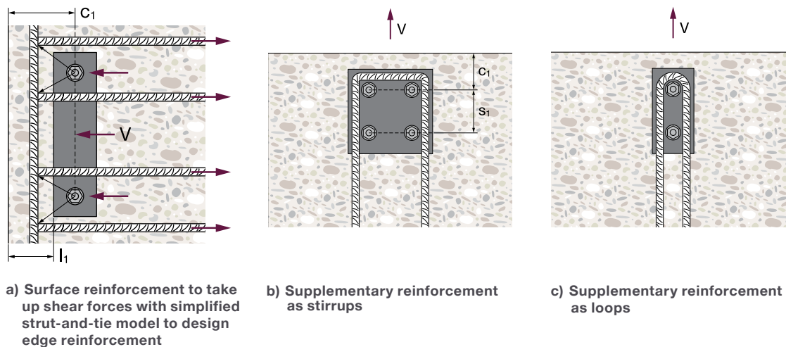
Fig. 6.22: Shear supplementary reinforcement for anchors
