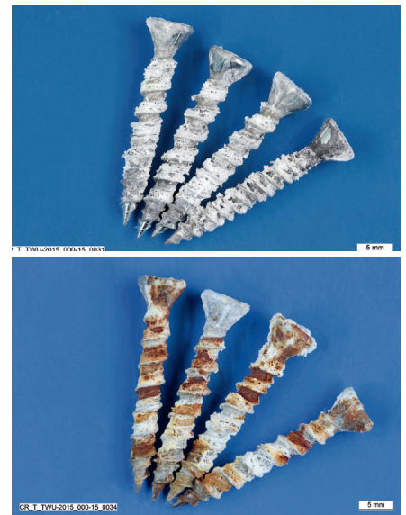
Fig. 14: Electrogalvanized screws with around 5 µm zinc coating after 48 h (up) and 96 h (down) in the salt spray test.
